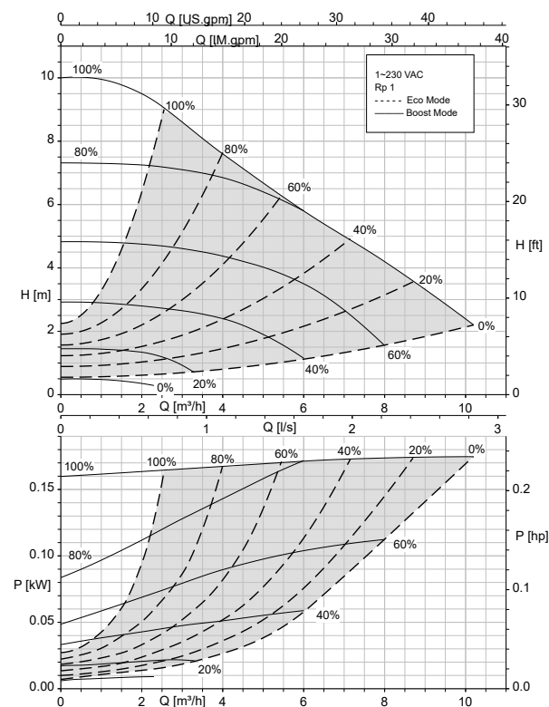
Calio 25-100 Open-loop Control, Eco Mode
