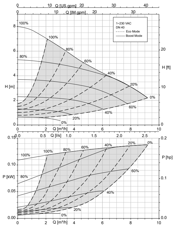
Calio 40-70 Open-loop Control, Eco Mode
