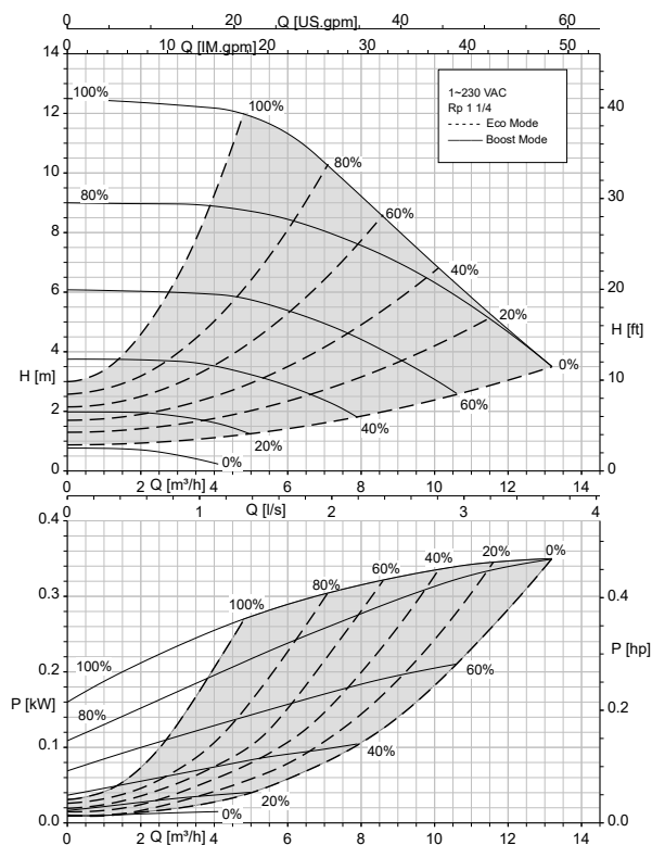
Calio 32-120 Open-loop Control, Eco Mode
