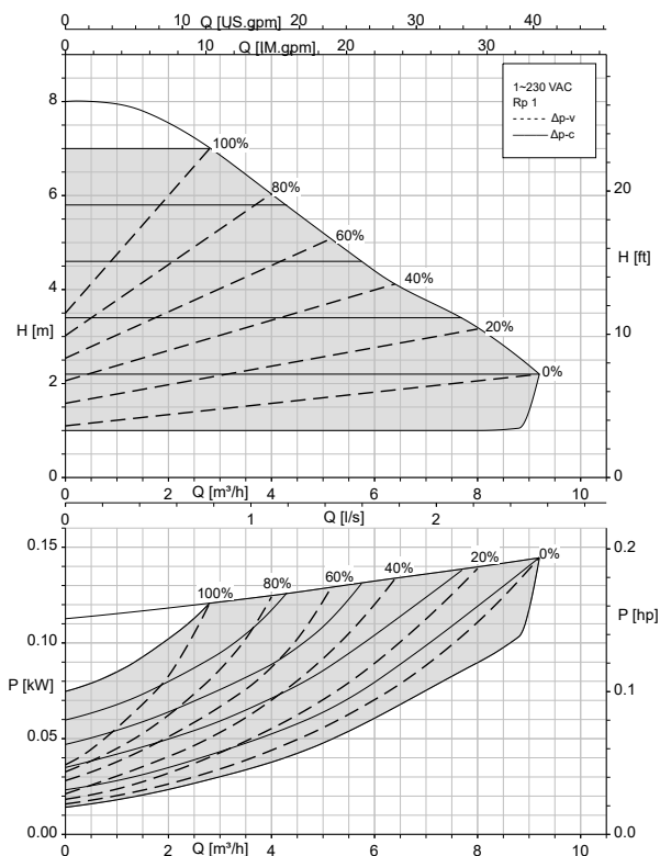
Calio 25-100 \Delta p_v , \Delta p_c
