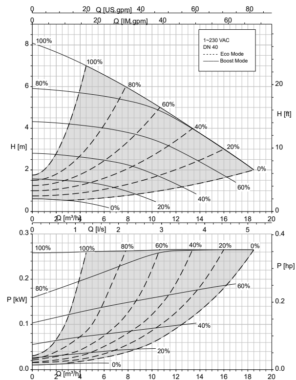
Calio 40-90 Open-loop Control, Eco Mode
