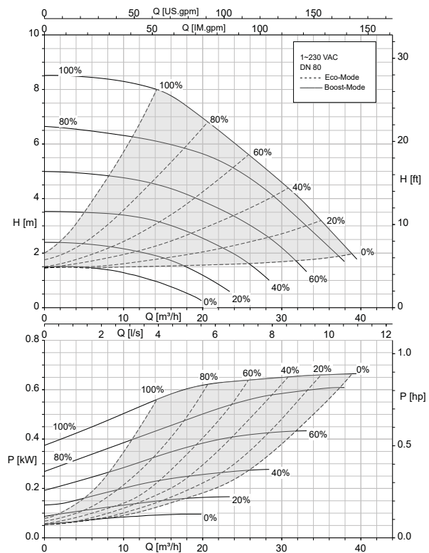
Calio 80-80 Open-loop Control, Eco Mode
