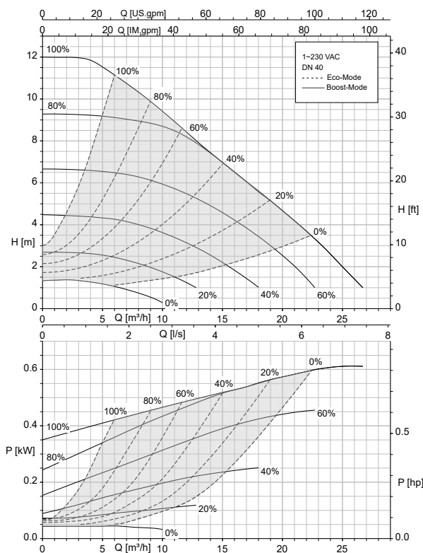
Calio 40-120 Open-loop Control, Eco Mode
