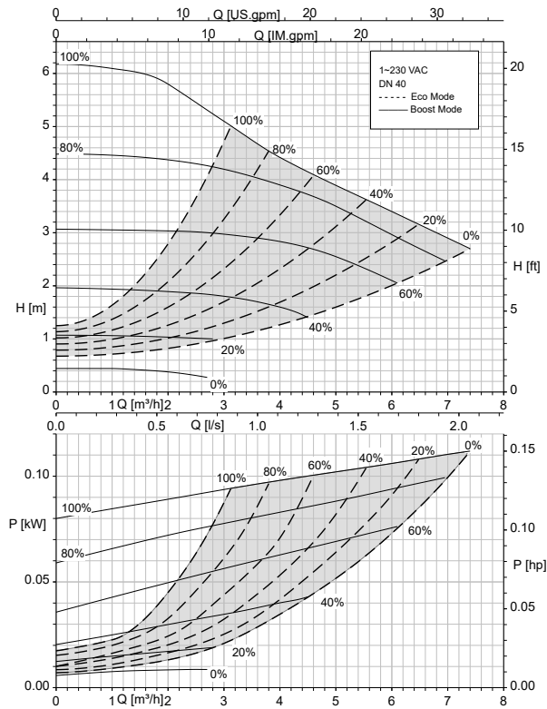
Calio 40-70 Open-loop Control, Eco Mode
