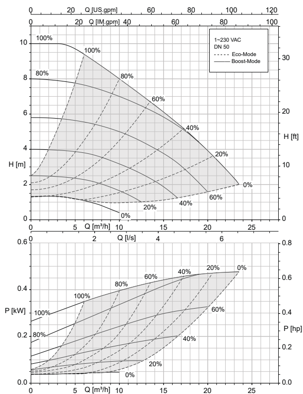
Calio 50-100 Open-loop Control, Eco Mode
