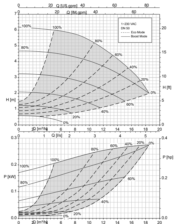
Calio 50-80 Open-loop Control, Eco Mode
