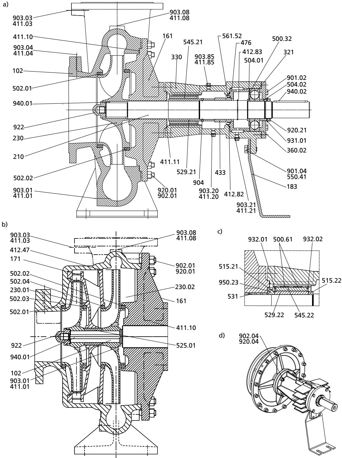
Fig. 6: a) Etanorm-RSY (single-entry) b) Etanorm-RSY (double-entry) c) SiC plain bearing d) back pull-out unit
