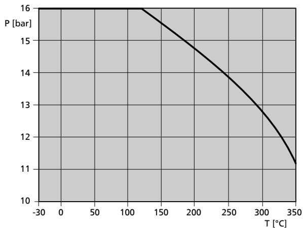
Fig. 1: Operating pressure limits and temperature limits 9)
