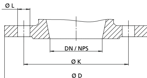
Fig. 9: Flange dimensions of Etanorm SYT
