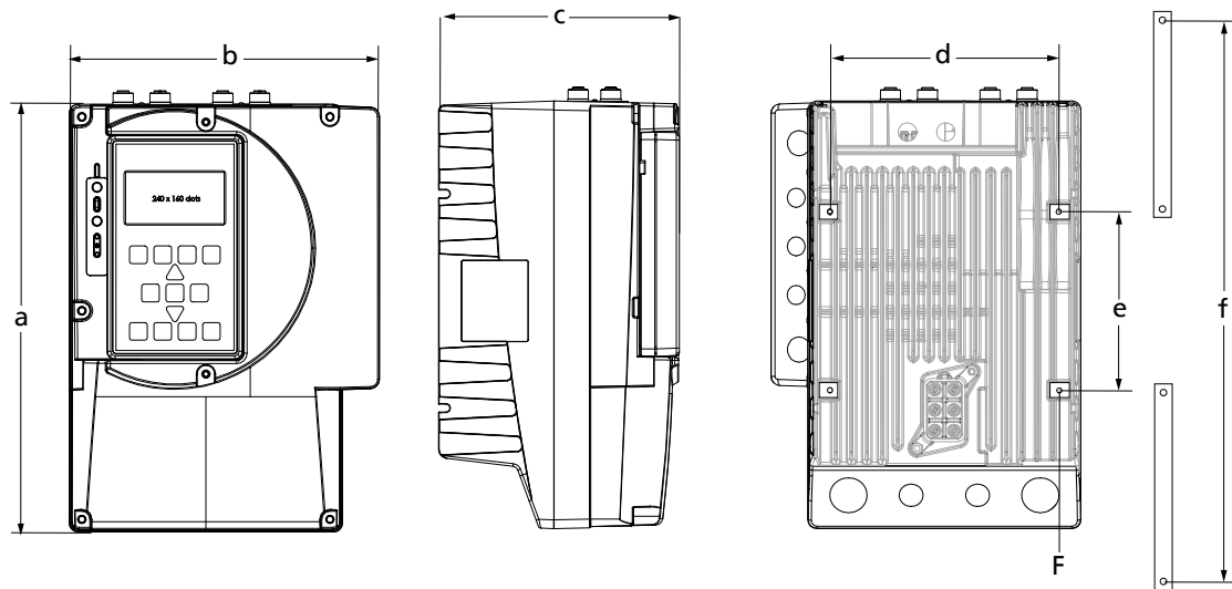
Fig. 3: PumpDrive 2 dimensions
