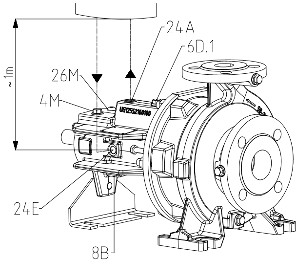
Auxiliary connections for double mechanical seal and monitoring equipment
