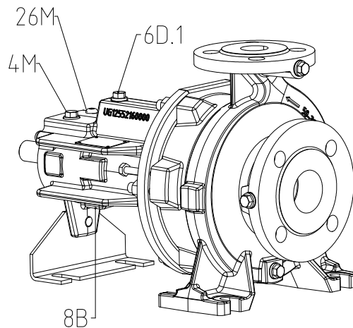
Auxiliary connections for single mechanical seal and monitoring equipment
