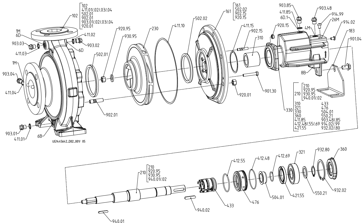
Fig. 10: Exploded view of an Etanorm SYT, bearing bracket WS_25_LS
