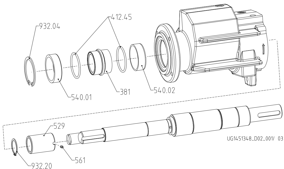
Fig. 15: Exploded view of Etanorm SYT, bearing bracket WS_35_LS with SiC plain bearing
