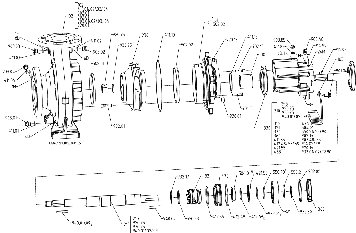
Fig. 13: Exploded view of an Etanorm SYT, bearing brackets WS_35_LS / WS_55_LS
