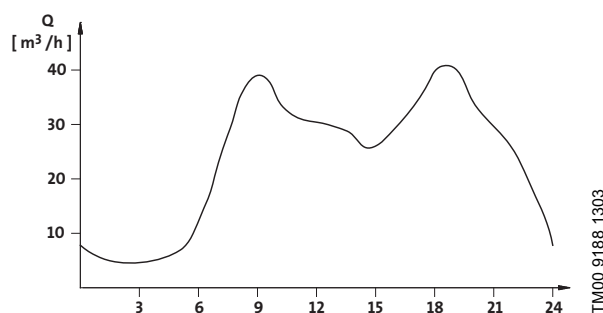
Fig. 18 Example of 24-hour consumption profile
