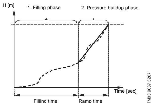
Fig. 9 Filling and pressure buildup phases
