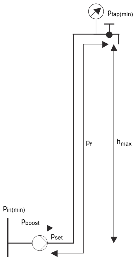
Fig. 17 Calculation of required outlet pressure
